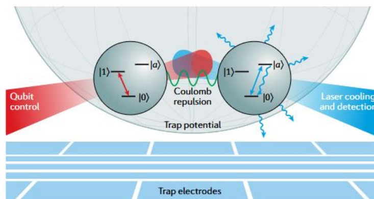
Fig. 1 | Quantum computing with trapped ions. At first glance, there are no materials in an ion-trap quantum computer, as shown in this schematic. The ions are held in an electromagnetic trap. Lasers or microwaves are used to control the internal states of qubits, |0\rangle and |1\rangle . The internal control and the Coulomb repulsion between ions combine to form conditional logic gates. Readout is performed by measuring laser-induced ion fluorescence using an auxiliary state |a\rangle . The laser-induced fluorescence is also used to cool the ions in preparation for quantum logic. The materials challenges arise when we consider how to generate the electromagnetic trap, deliver the control laser beams and detect the ions' fluorescence.
